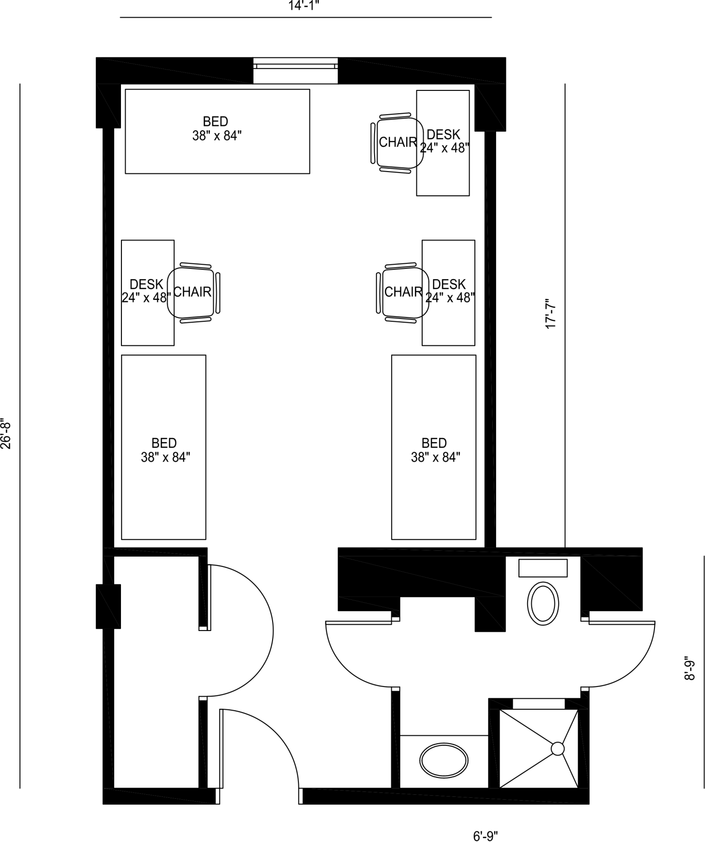
VAUGHN CENTER - FLOORPLAN L
